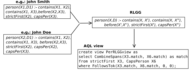
Figure 3: Relative Least General Generalization
