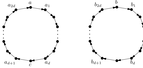
Fig. 1. Instance I of Corollary 4.8.
