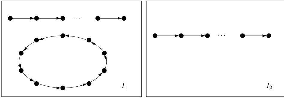
Fig. 3. Instances I_1 and I_2 of Theorem 6.6.
