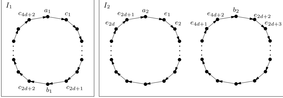
Fig. 2. Instances I_1 and I_2 of Corollary 4.9.
