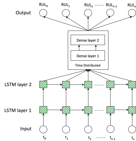
(b) LSTM many-to-many model
